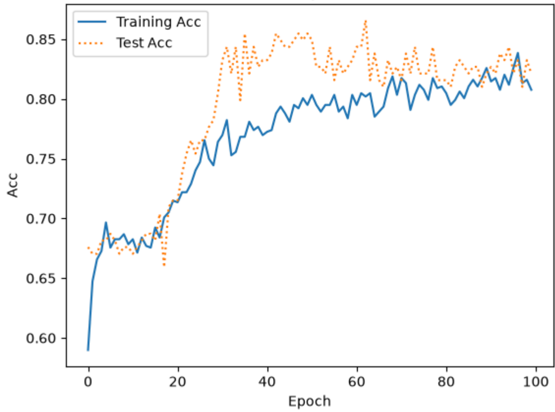
Accuracy Curve
